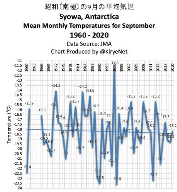
Figure 9: Antarctica 1960->2020
