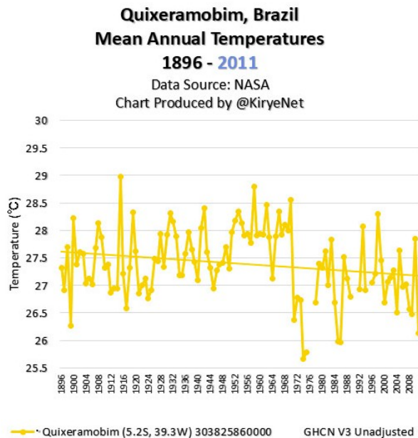
Figure 7: Brazil - 1896 -> 2011
