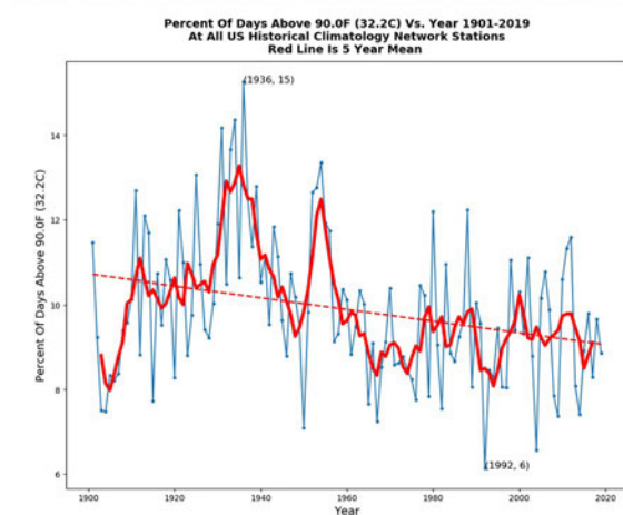
Figure 12: USA 1901-> 2019
