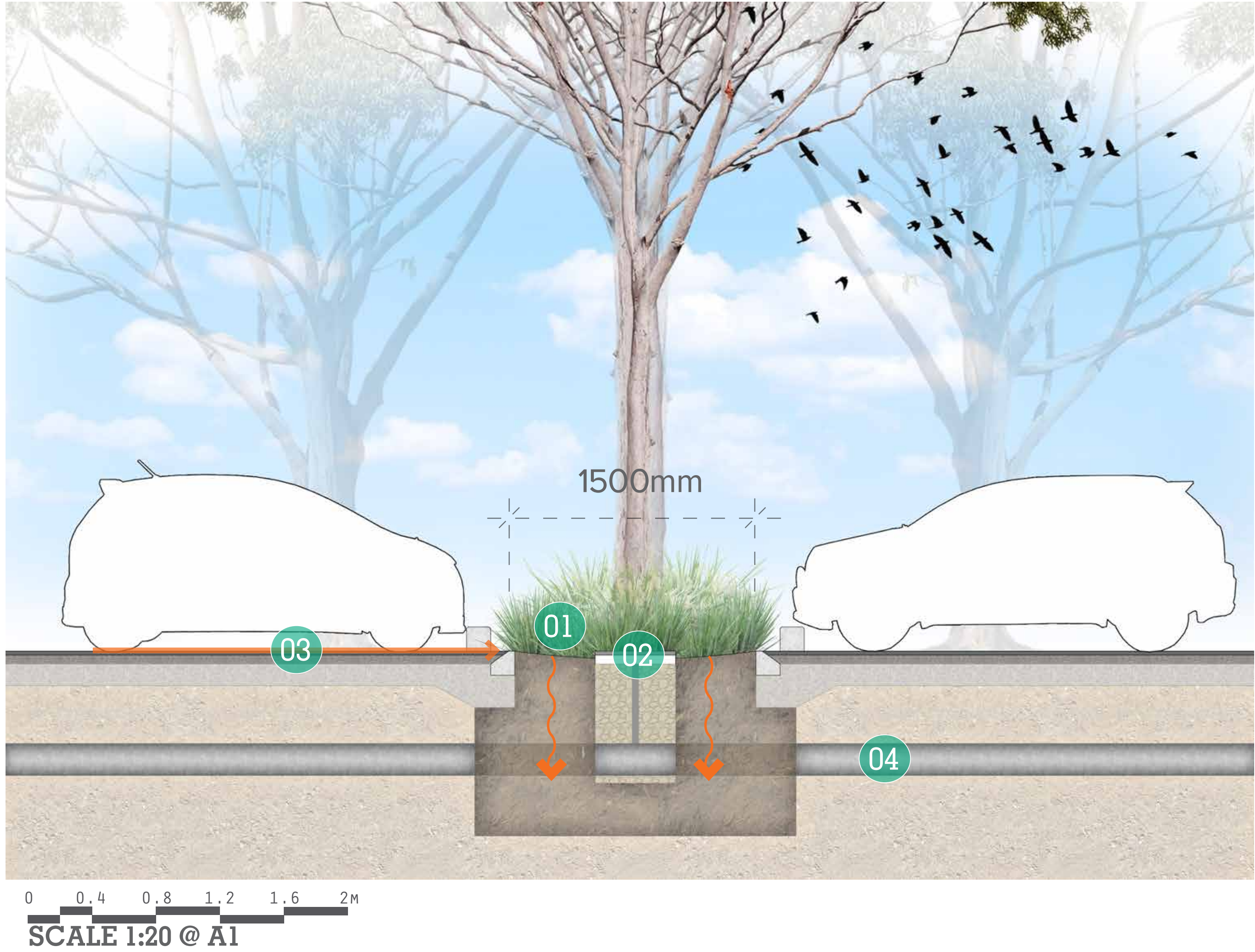
CAR PARK SECTION DD
