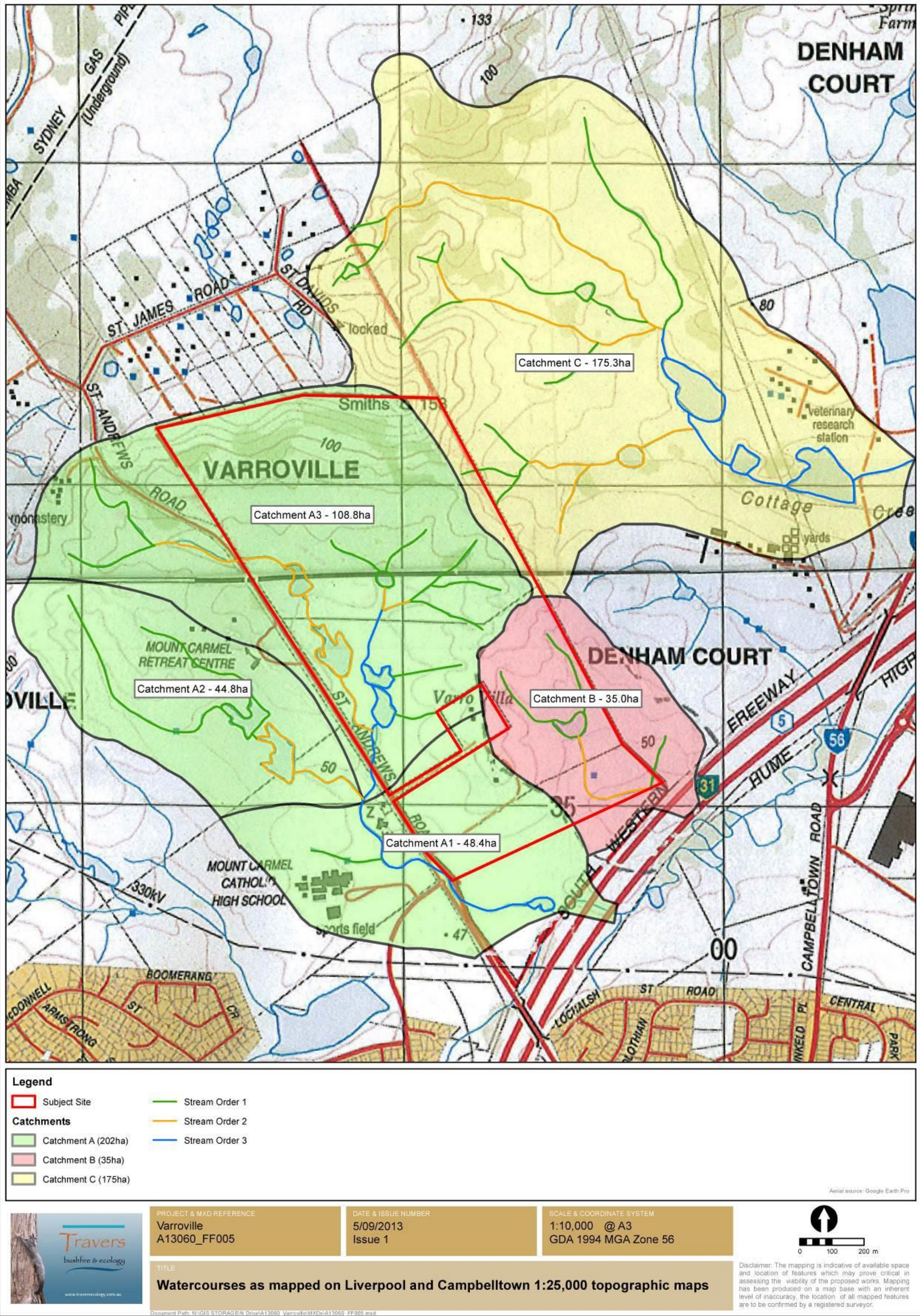
Figure 4 – Catchments, mapped watercourses and stream order (Liverpool and Campbelltown 1:25000 topographic maps)
