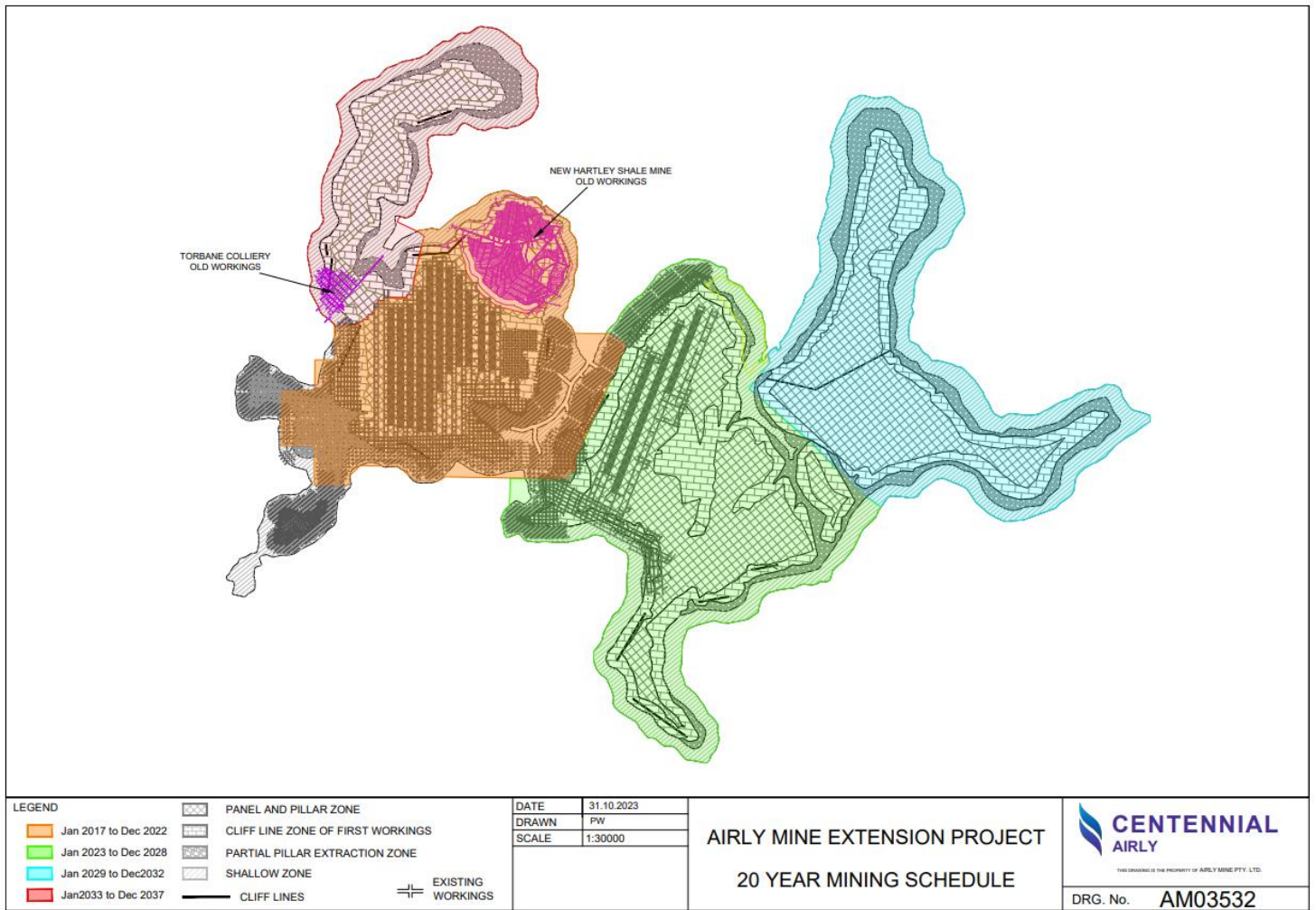
Figure 3A: Mining schedule
