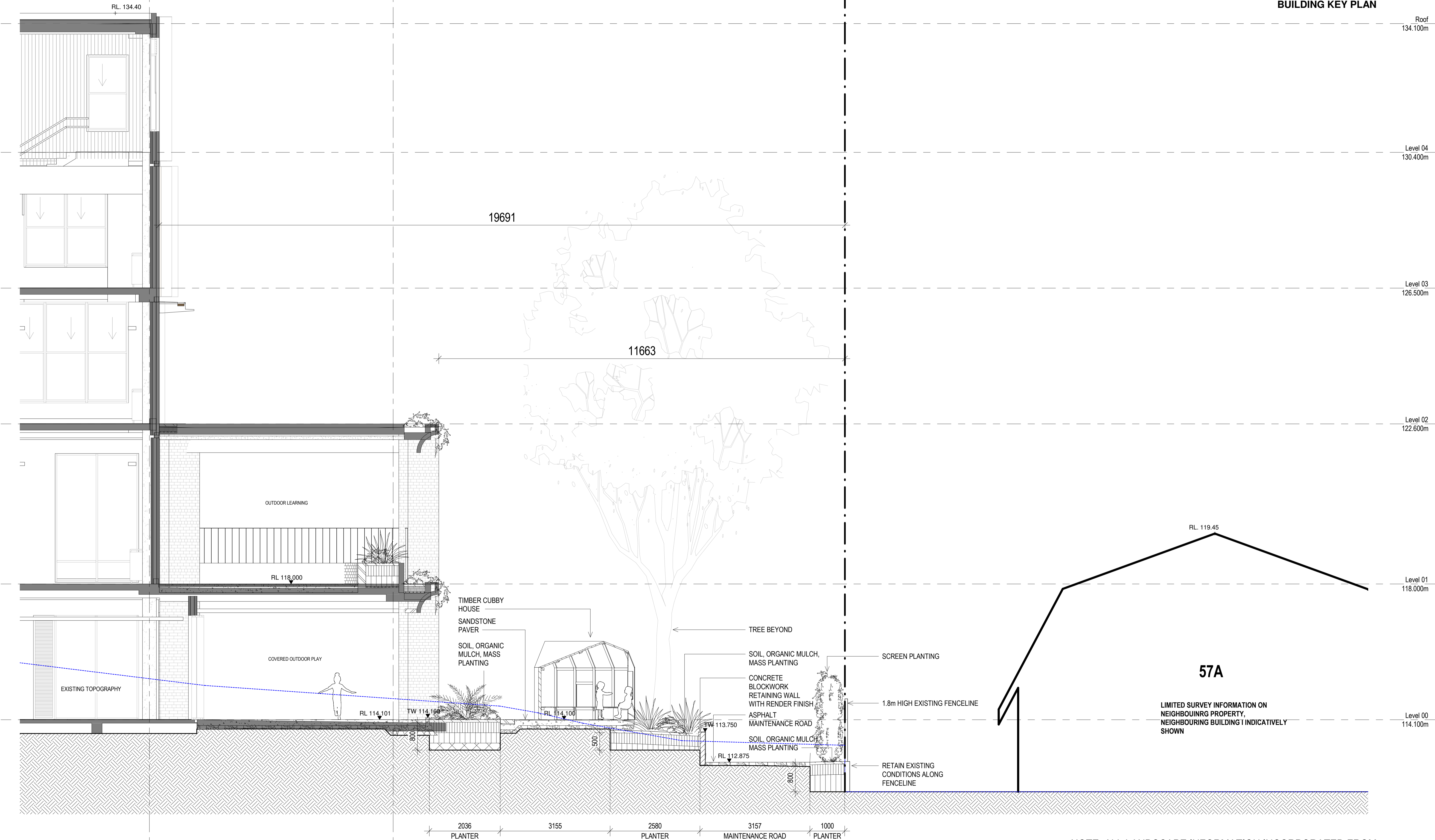
SKETCH 91 - 1:50 REAR SETBACK SECTION 01 - 57A
