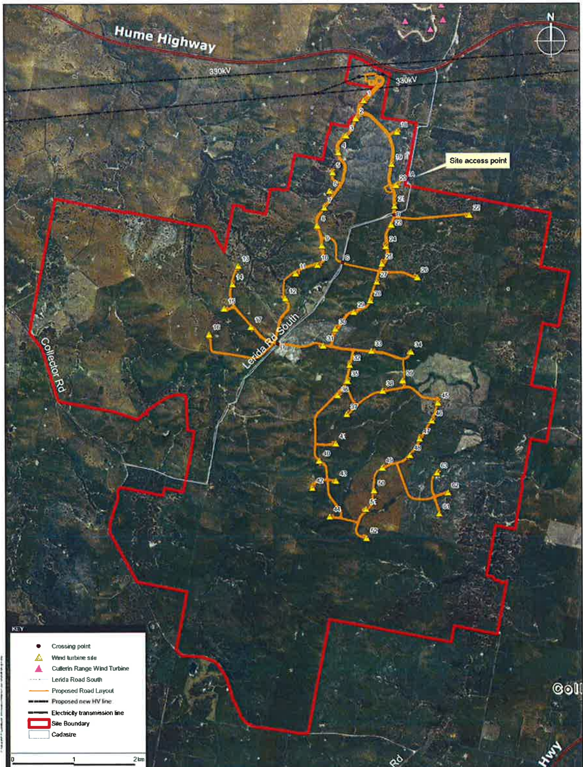
Figure 2: Project layout
